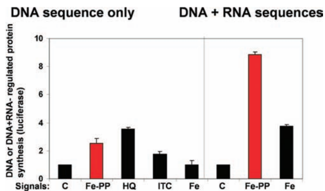
Figure 1. Dual regulation of mRNA and DNA by heme–repressor (bach 1 or IRP) interactions. Luciferase activity, encoded in plasmids under the control of the human ferritin L DNA–ARE promoter or the human ferritin L DNA–ARE promoter plus the mRNA–IRE 5′UTR regulator (promoter), was measured in HeLa cells as described in ref 59. Antioxidant response inducers: Fe-PP, Fe-protoporphyrin IX (heme); HQ, t -butylhydroquinone; ITC, 4-methylsulfanylbutyl isothiocyanate (sulforaphane; iron inducer is ferric citrate (1:10)), 59 and the data are from ref 59 with the error as the standard deviation.
