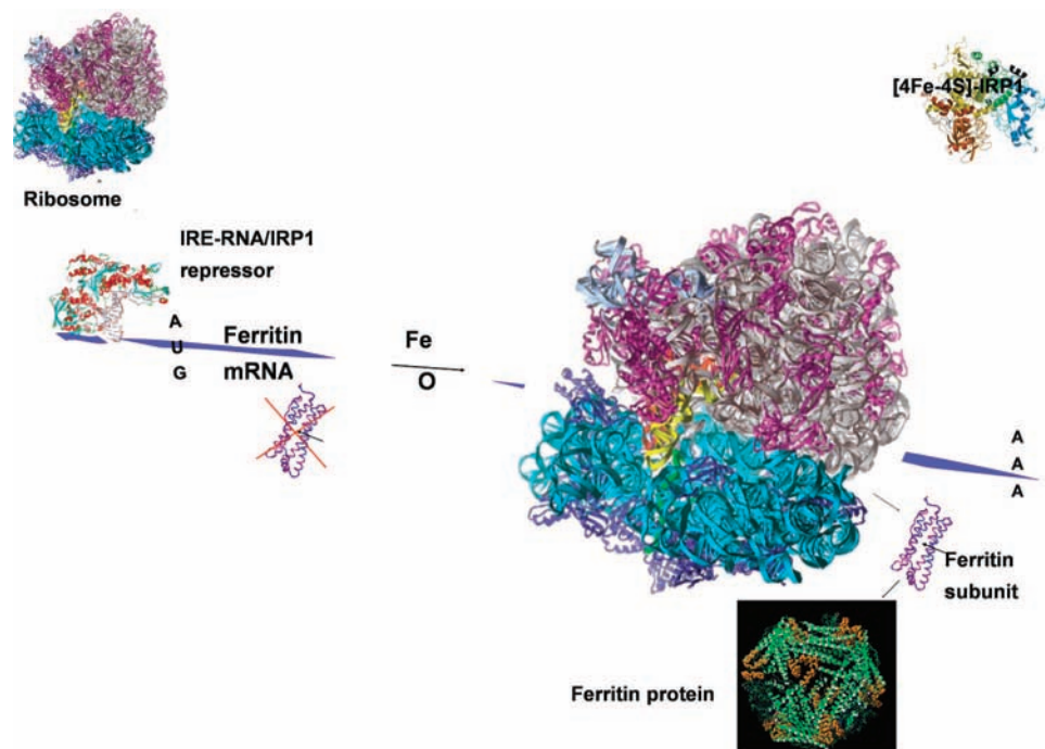
Figure 3. Model for IRE/IRP-regulated translational control. Structures incorporated into the illustration are taken from IRE-RNA/IRP complex, 97 ribosome, 155 ferritin subunit, 156 and ferritin nanocage. 157
