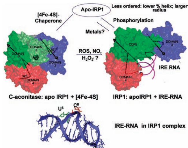
Figure 2. Structure of an IRE RNA and complexed with IRP1. Data are modified from ref 97; apo-IRP has not been crystallized to date and appears to have disordered regions. 154 The ribbon diagram of the IRE-RNA used PDB file 2IPY.
