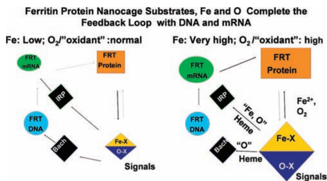
Figure 4. Links between oxygen and iron homeostasis through ferritin: The Fe/O feedback loop. Frt = ferritin; IRP = iron regulatory protein, binds ferritin IRE–RNA; IRE = iron responsive element; bach-1 = a transcription factor that binds ARE–DNA; ARE = antioxidant response element.
